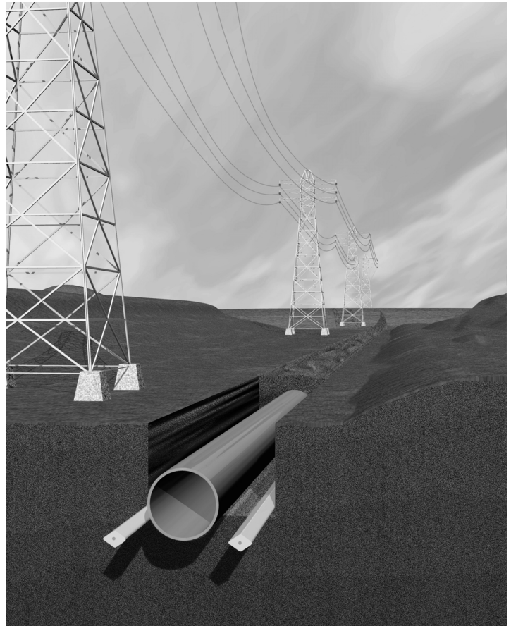
Figure 1 – Plattline used for AC mitigation
